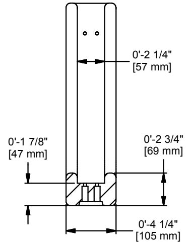
CROSS SECTION
