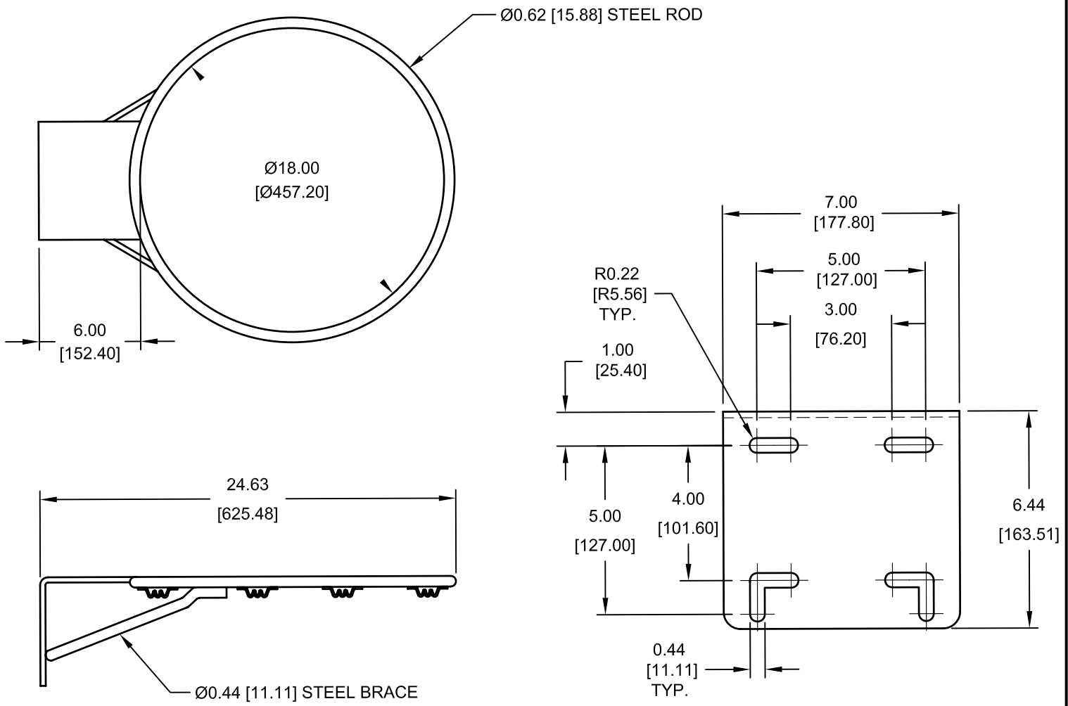
MOUNTING PLATE VIEW SCALE 2:1
