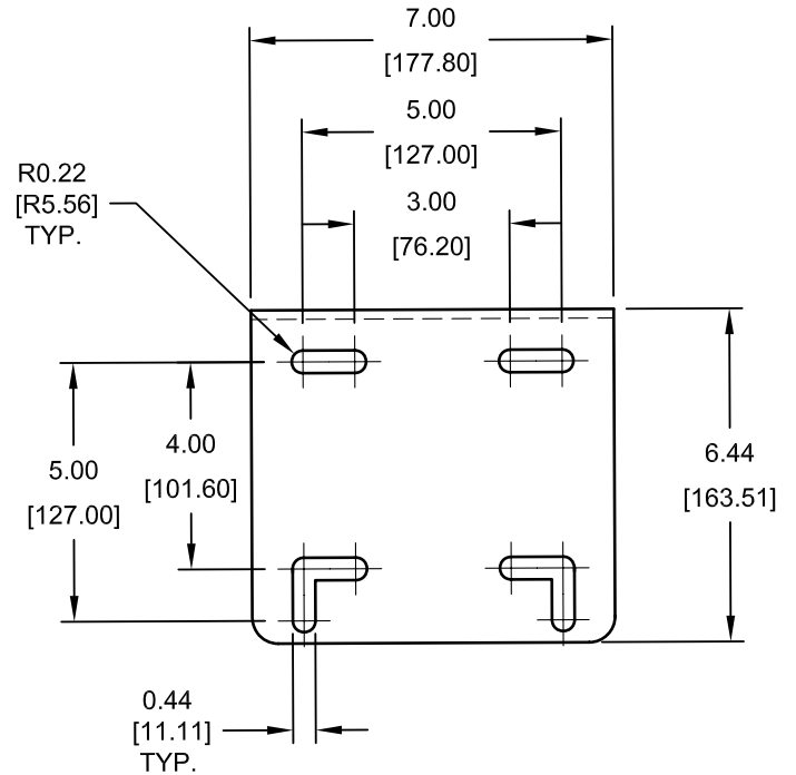
MOUNTING PLATE VIEW SCALE 2:1
