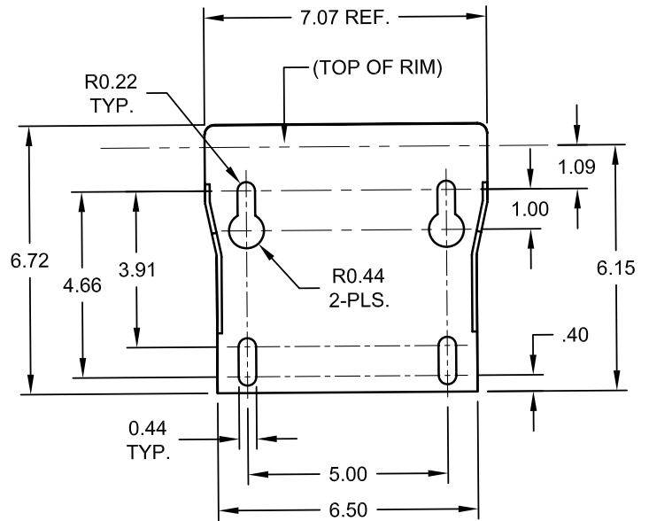
MOUNTING PLATE VIEW SCALE 2:1
